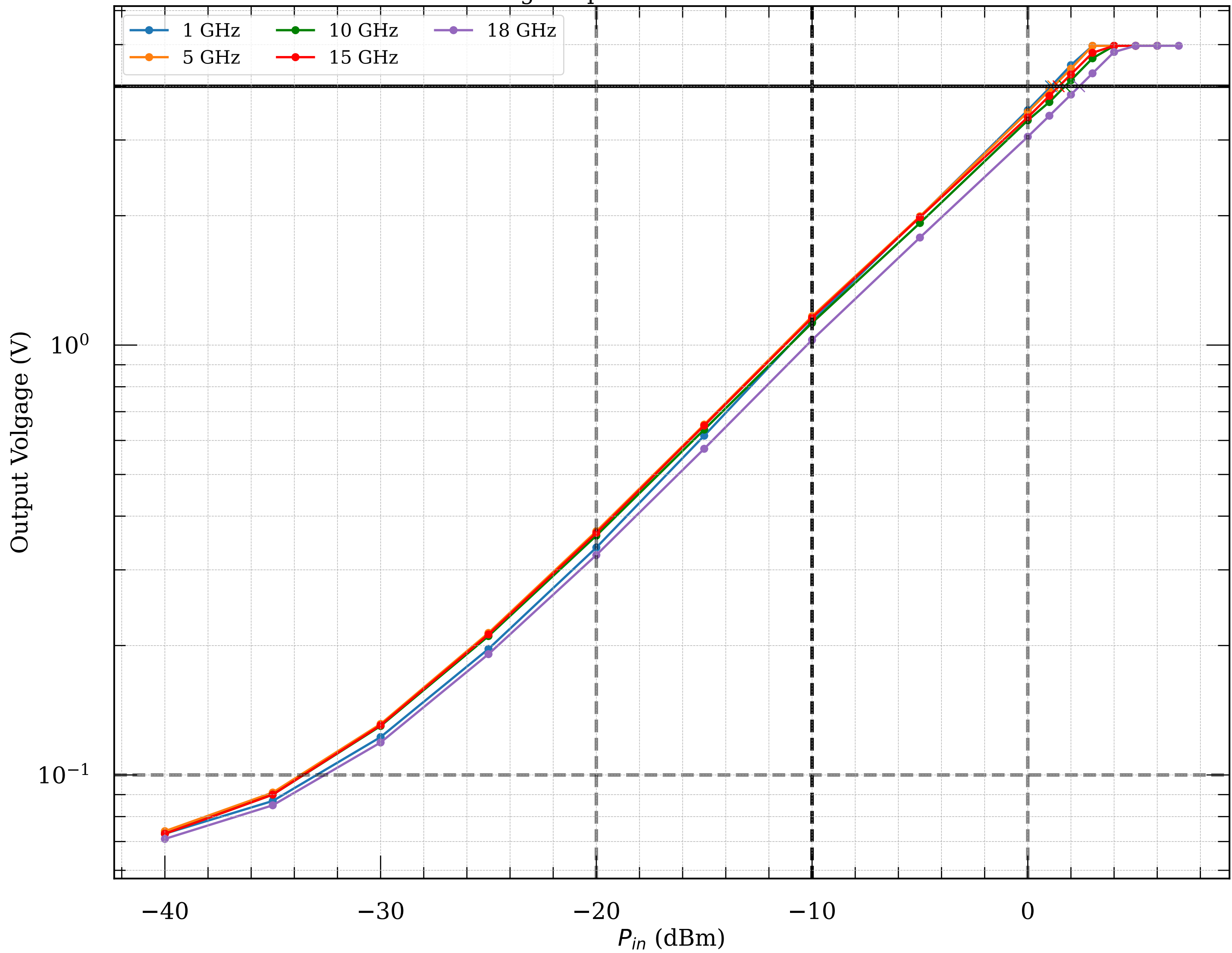
Measured voltage-to-power curve of detector module098
